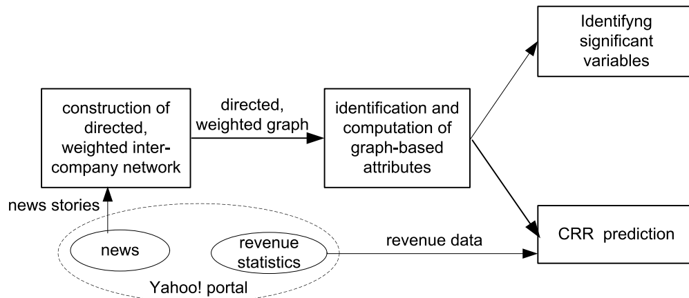
Figure 4. Diagram of methodology and analysis approaches
