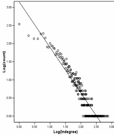
Figure 3. Node indegree (NID) distribution
