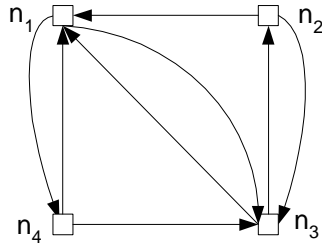
Figure 1. Directed graph
